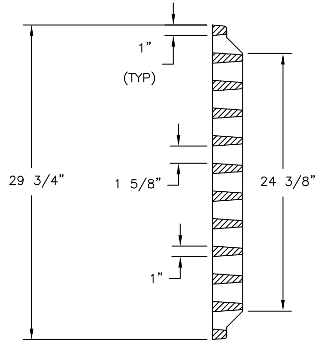
GRATE SECTION
