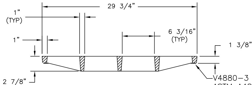
GRATE SECTION
